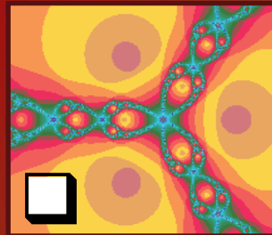
Newton fractal ( Z^n - 1 ) \geq order 3
